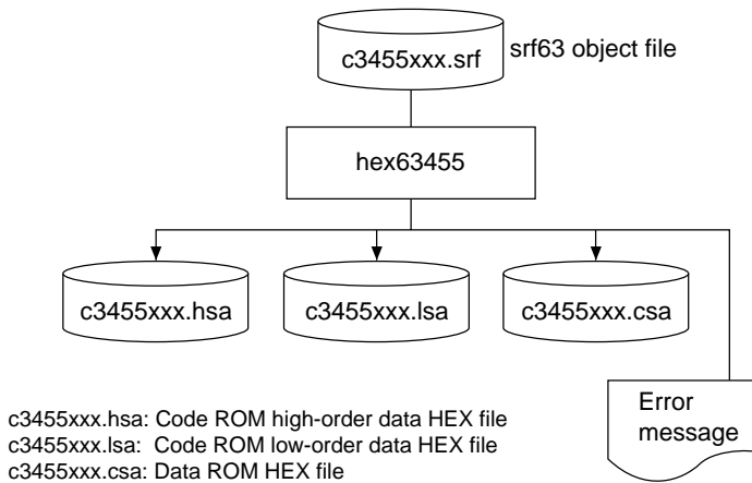
Fig. 2.2.1 hex63455 execution flow
