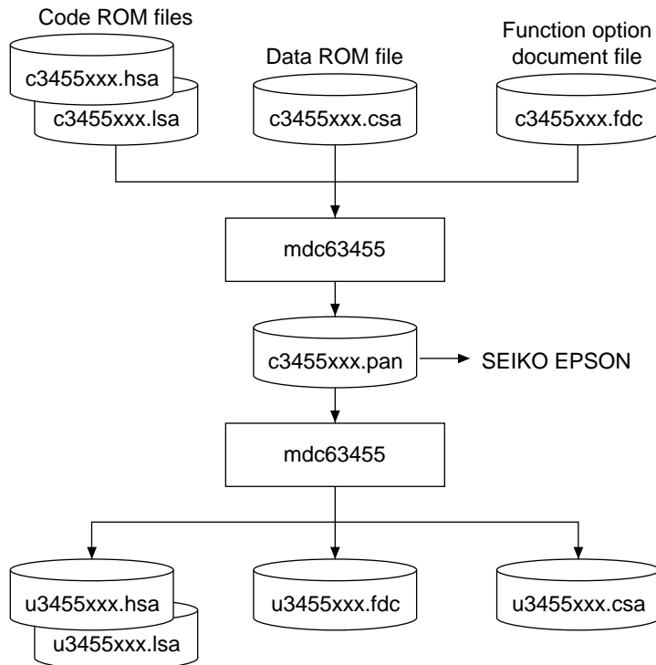
Fig. 4.2.1 mdc63455 execution flow
