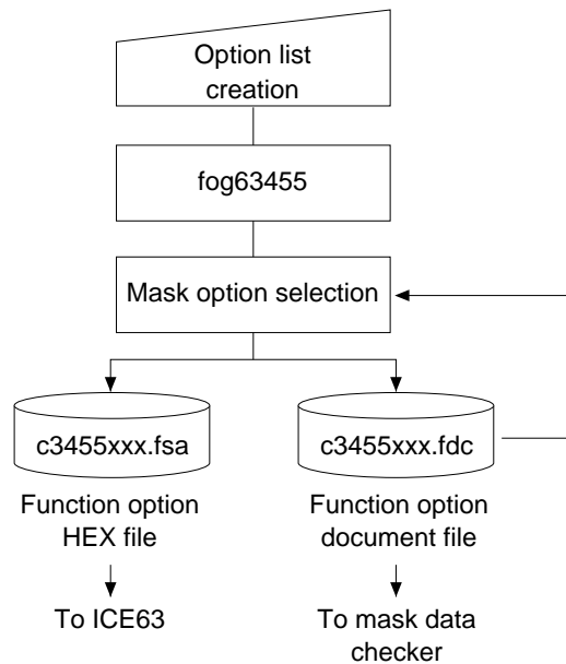
Fig. 3.2.1 fog63455 execution flow
