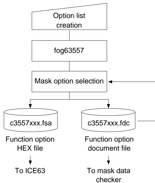
Fig. 3.2.1 fog63557 execution flow
