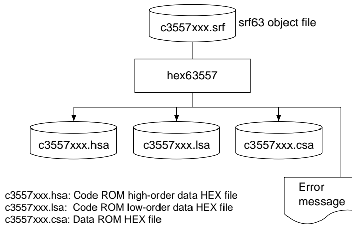
Fig. 2.2.1 hex63557 execution flow
