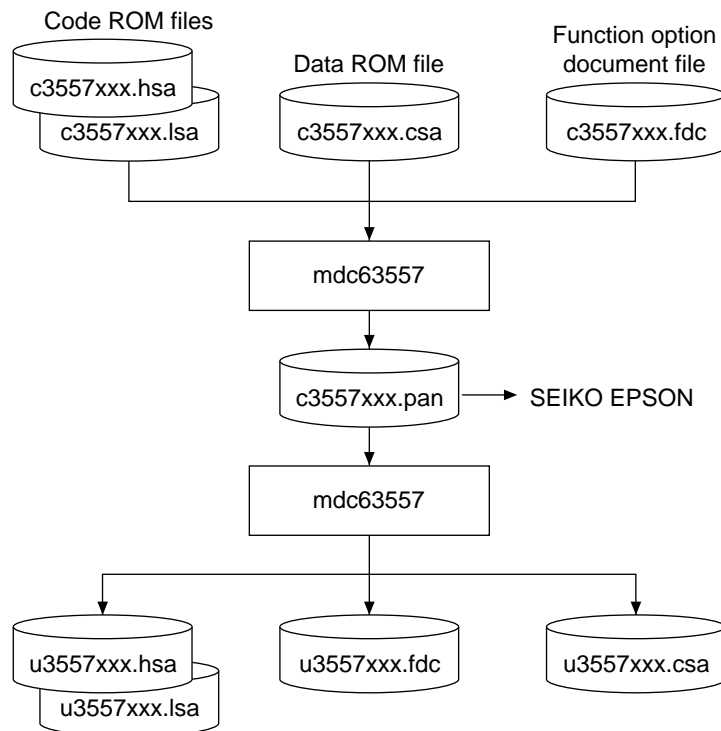
Fig. 4.2.1 mdc63557 execution flow
