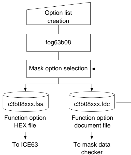
Fig. 3.2.1 fog63b08 execution flow
