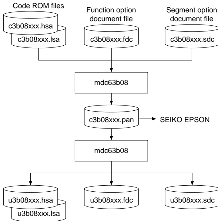
Fig. 5.2.1 mdc63b08 execution flow
