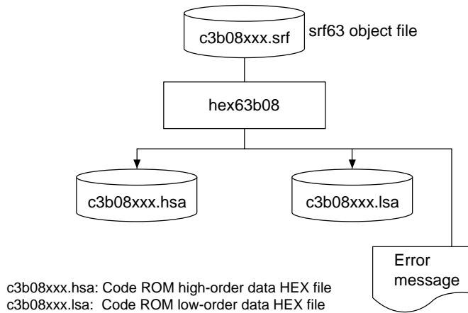
Fig. 2.2.1 hex63b08 execution flow
