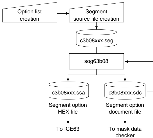
Fig. 4.2.1 sog63b08 execution flow
