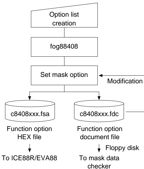
Fig. 3.2.2.1 fog88408 execution flow
