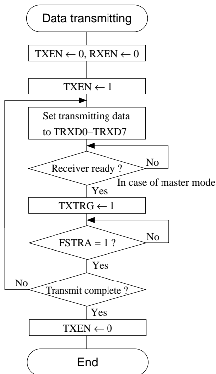
Fig. 5.8.6.2 Transmit procedure in clock synchronous mode
