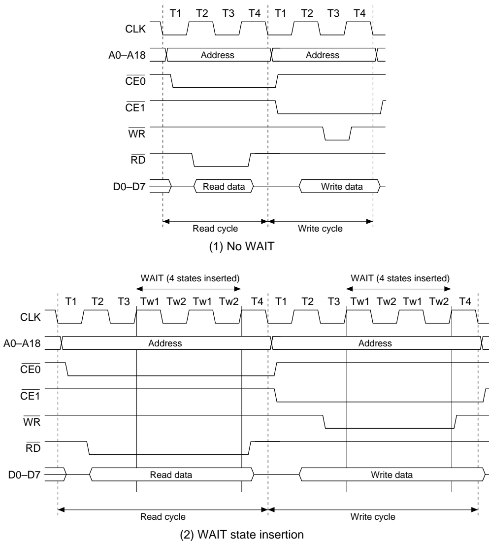
Fig. 3.6.5.1 Memory read/write cycle
